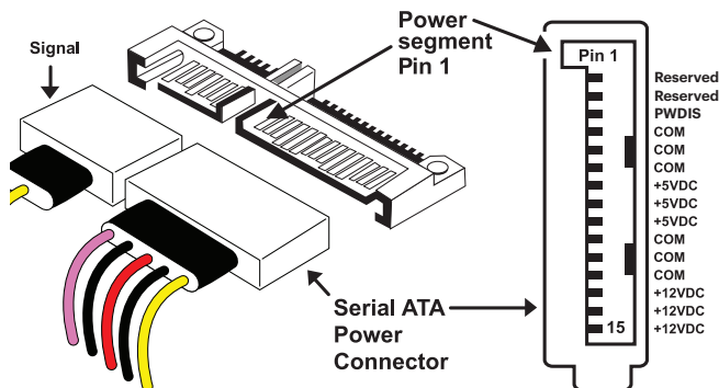
Figure 2: A typical SATA connector that supports Power Disable (PWDIS)
